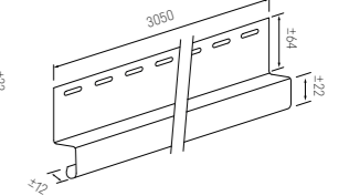
SVP 19 Facade flashing large
