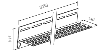
SV 11.5 Lower ventilation trim
