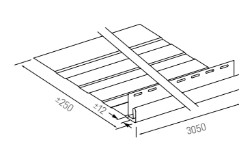
SVP 19 Facade flashing large
