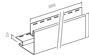
SVP 12 Outside corner
