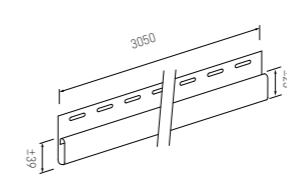
SVP 18 Joint trim
