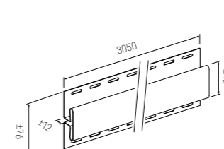
SVP 18 Joint trim
