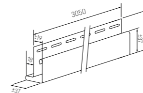
SVP 17 Facade flashing small
