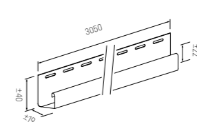
SVP 19 Facade flashing large
