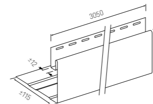
SVP 17 Facade flashing small
