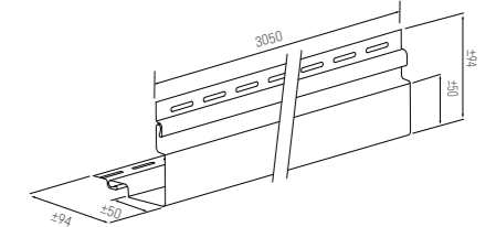
SVP 12 V Outside corner for vertical installation
